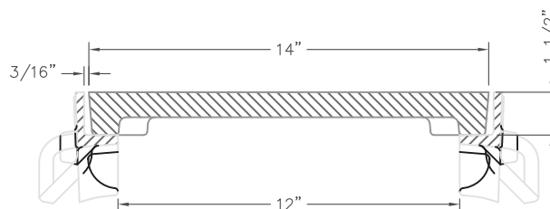
R-4990-DX TYPE "D" LID w/ TYPE "B" FRAME TYPICAL SECTION (SCALE: 1/4"=1")
